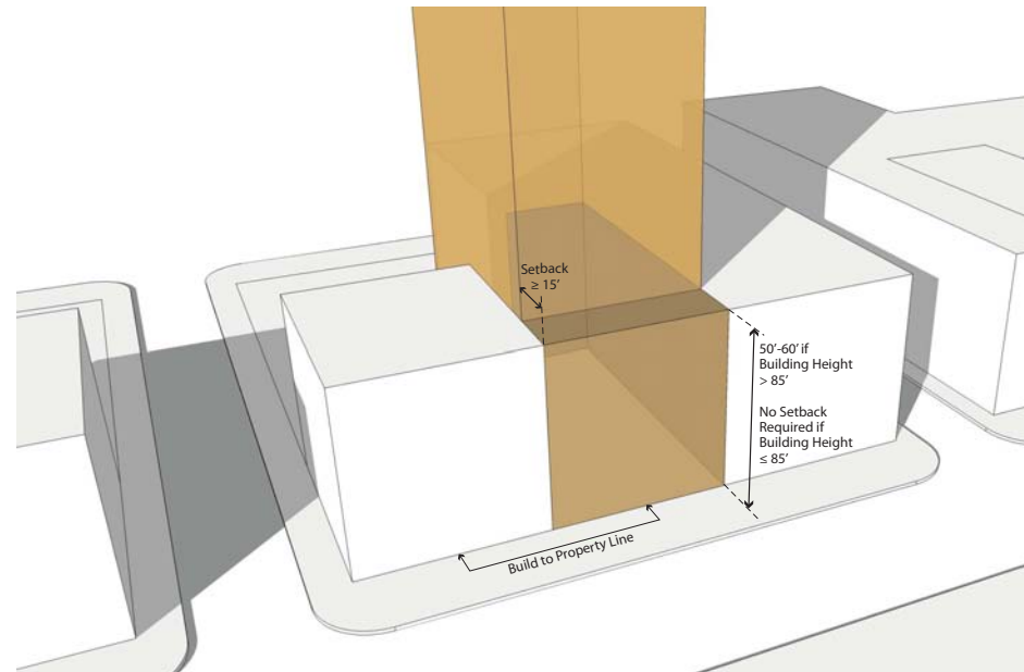
Streetwall guidelines for buildings within the 2nd/New Montgomery Conservation District.
