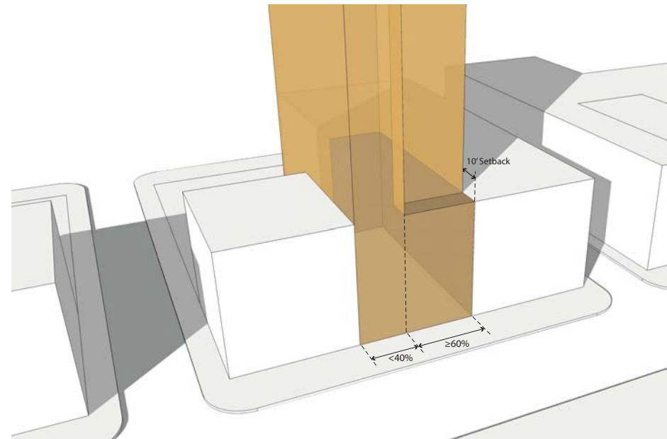
Streetwall guidelines for buildings taller than 150 feet.
