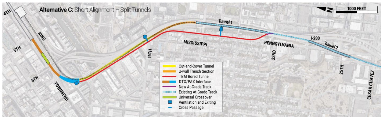
Figure 5-5. Fire/Life Safety Features for Short Alignment – Split Tunnels
